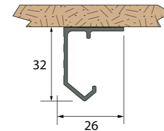
Rail 30 (1.94 - 3 m)
