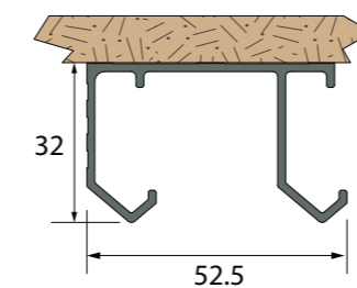
Rail 40 (1.94 - 3 m)
